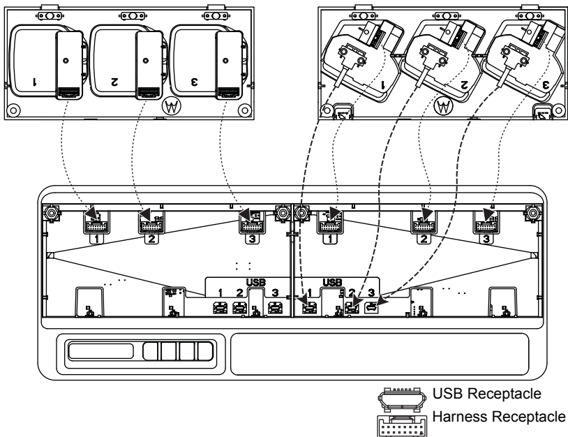
Figure 27: Securing HW001384A01/HW001385A01/HW001386A01/ AS000063A01 Charging Pockets to Multi-Unit Charger Base
