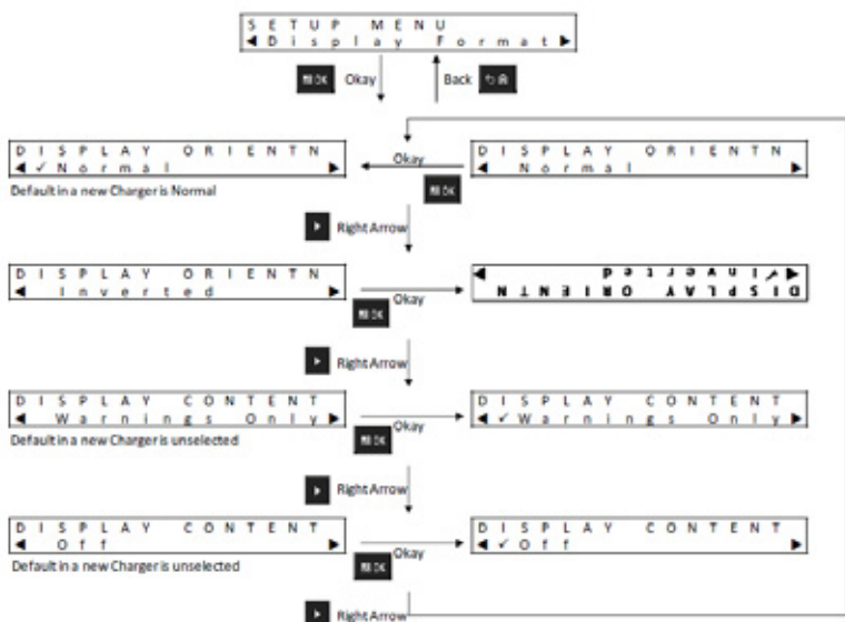
Figure 10: Display Format Menu
