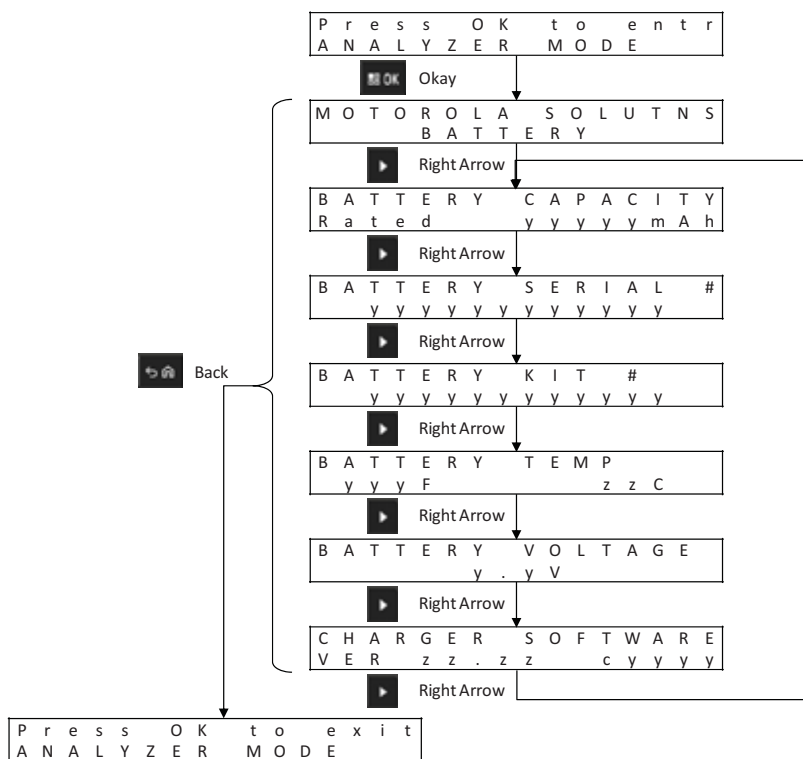
Figure 17: Other Motorola Solutions Battery Menu
