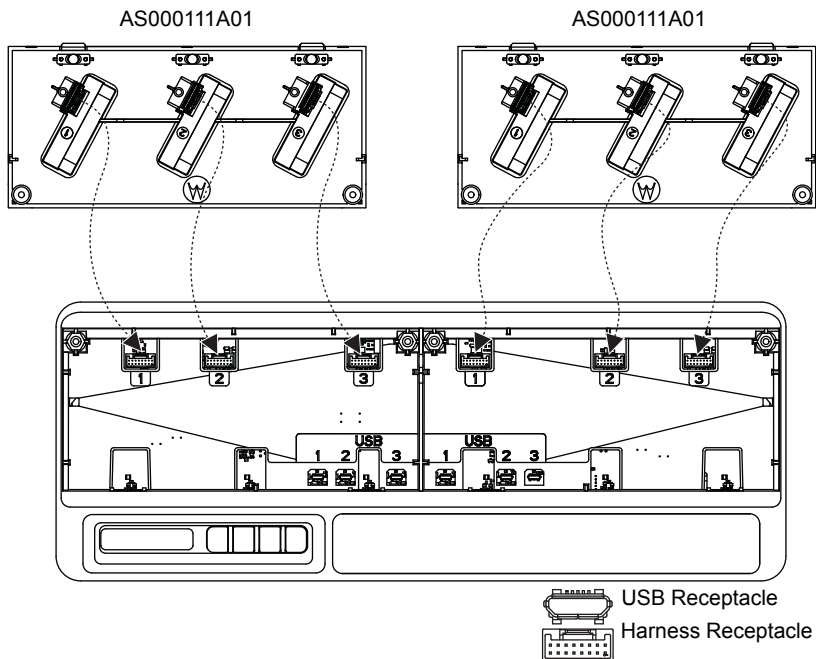
Figure 28: Securing AS000111A01 Charging Pockets to Multi-Unit Charger Base
