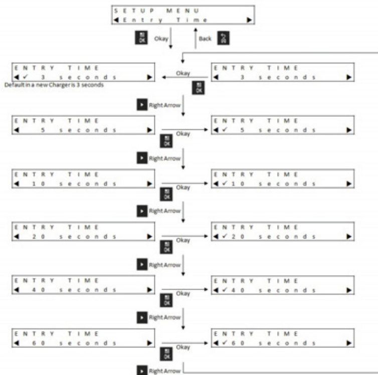
Figure 13: Entry Time Menu
