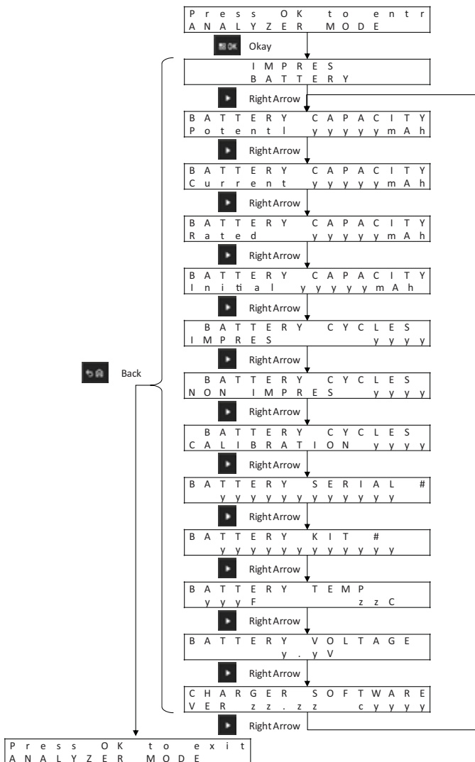
Figure 16: IMPRES Battery Menu
